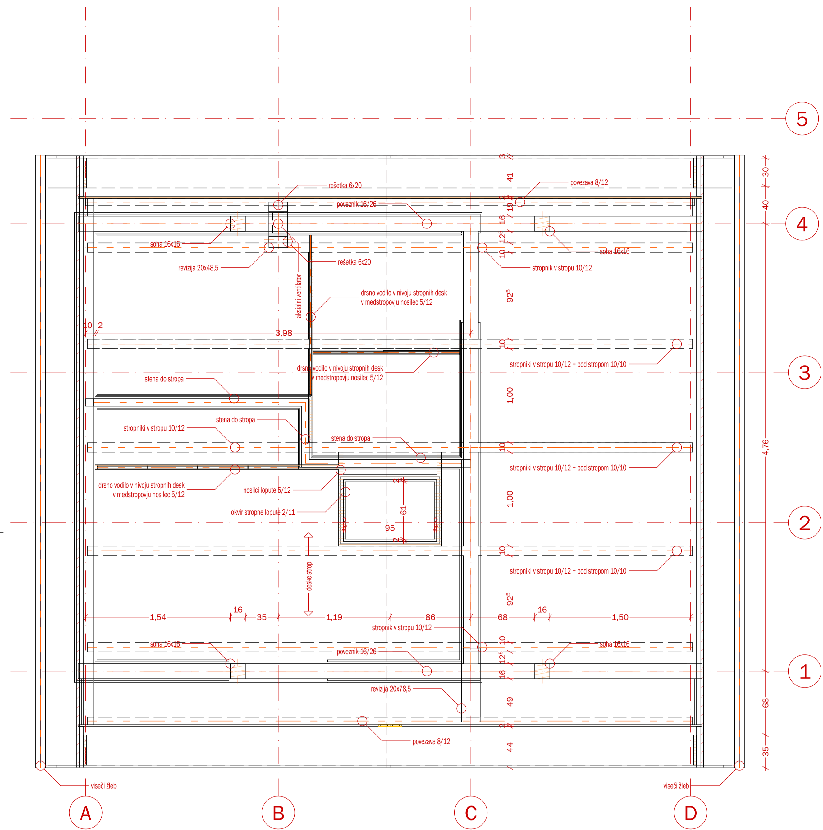
1. strop novo 1:25
